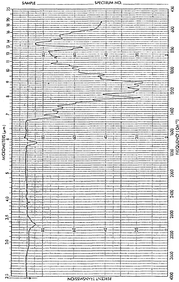
Figure 7 - Infrared of \text{CF}_2\text{BrCFClCH}_2^*(\text{CF}_3)\text{CH}_2^*\text{CHBrCF}_3
